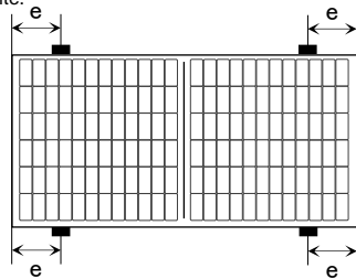
Figure2.Maximum load by Clamping on Longer Frame
