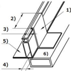
Figure1. Clips (Clamps) requirement 1) Clip: Al alloy, 3mm Min. thickness 2) Catch length (50mm Min.) 3) Covering depth (7mm Min. on the frame) 4) Supporting depth (10mm Min.) 5) Frame (applicable to all frame sections) 6) Array rail (applicable to parallel or crossed mounting)
